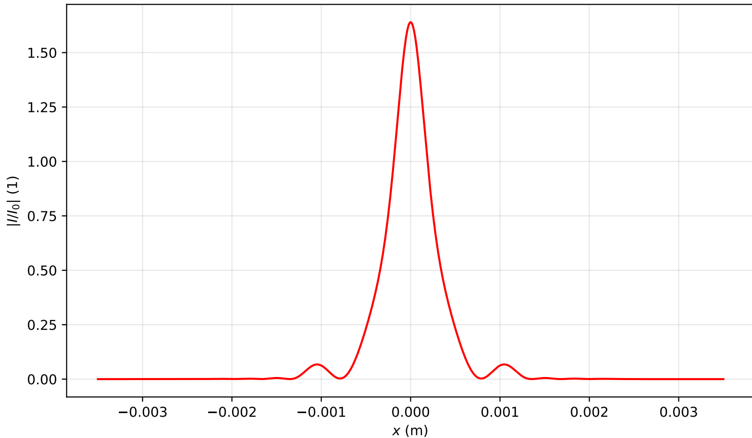
Intensity profile I(x, y = 0, z = 1.911)/I_0 , P_{in}=2.0P_{cr} , artificial time
